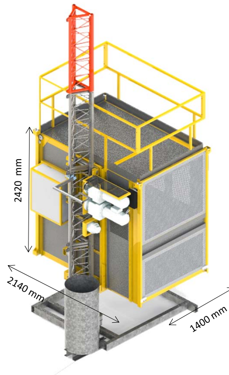
Cabin Ext. Dimensions
